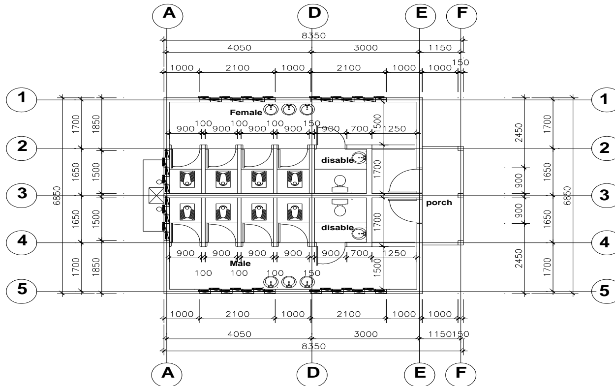
GROUND FLOOR PLAN 10-SEATER POURFLUSH TOILET
